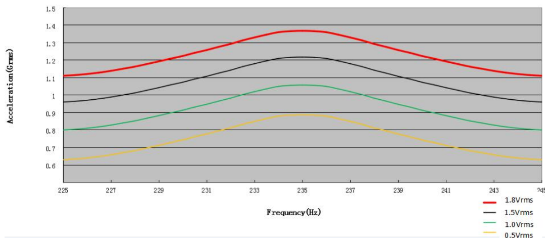
Figure 2. Frequency Response
