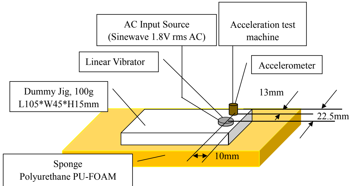
Figure 1. Test method
